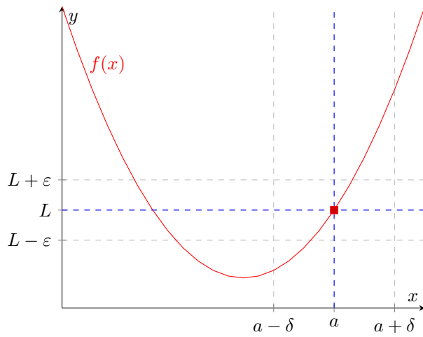
Figure 1: epsilon-delta
